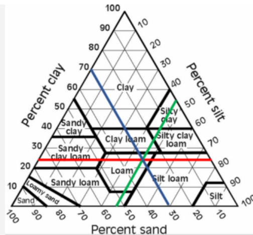
1. Soil texture triangle to estimate the soil type for the site
